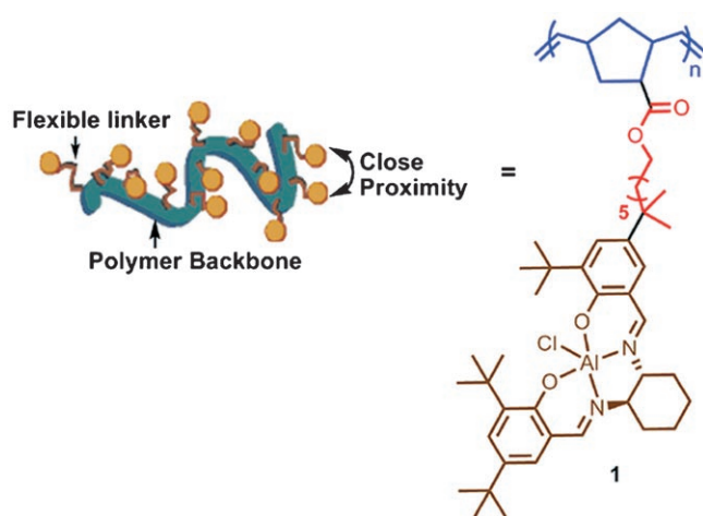
Figure 1. Schematic representation of the research design and catalyst 1 employed in this study.
