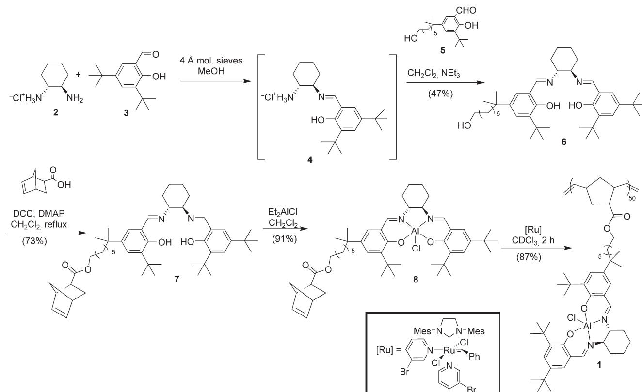
Scheme 1. Synthesis of polymeric catalyst 1 .
